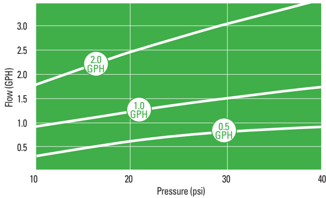
FLOW RATE VS. PRESSURE
