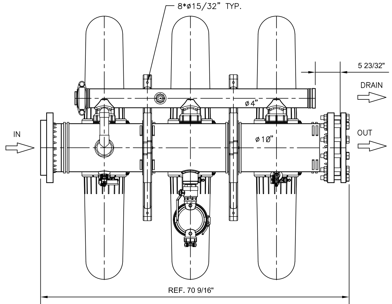
00 APOLLO TWIN 3 UNIT NOT TO SCALE
