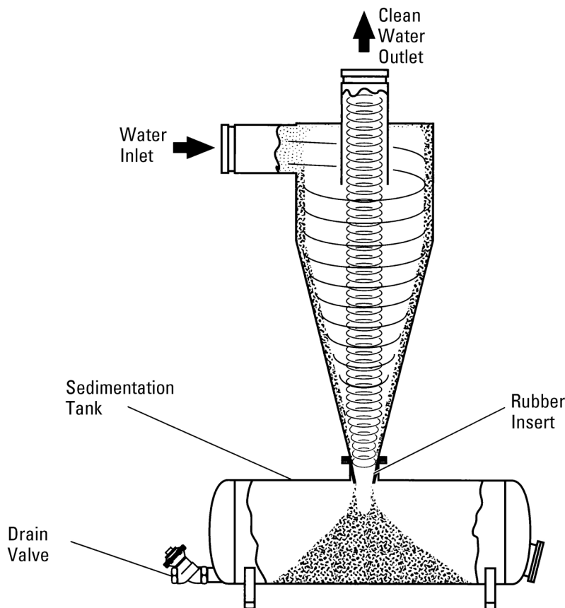
Hydrocyclone Flow and Mode of Separation
