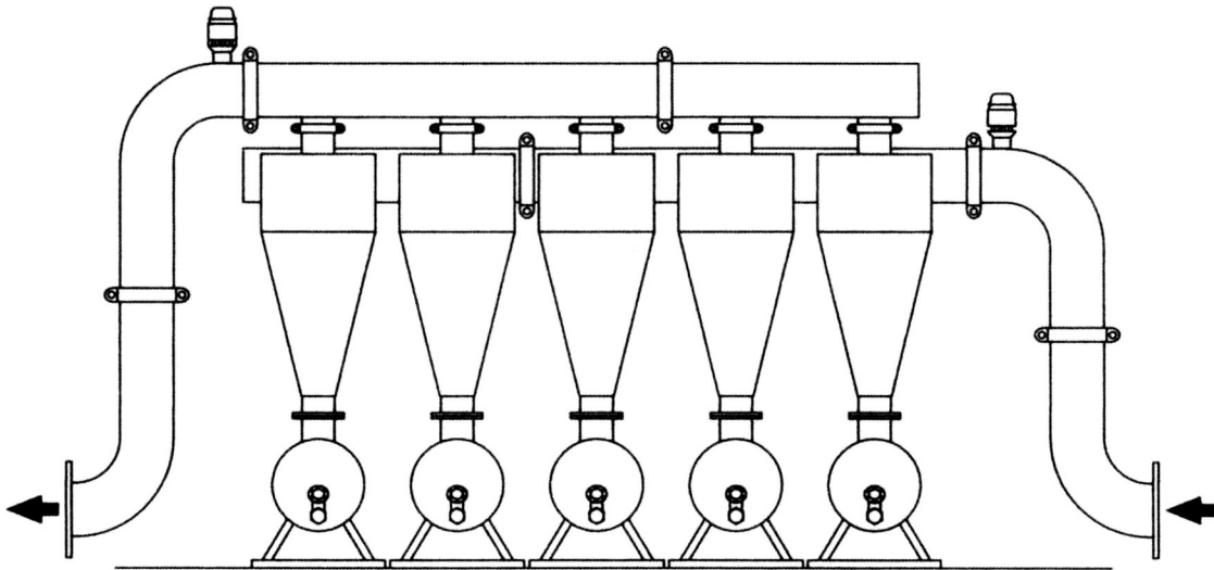
Multiple Hydrocyclone and Sedimentation Tank Installation
