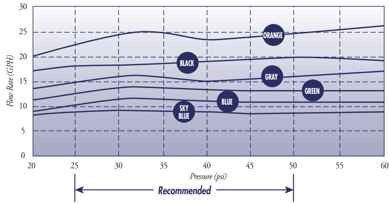
SUPERNET JET Flow vs. Pressure
