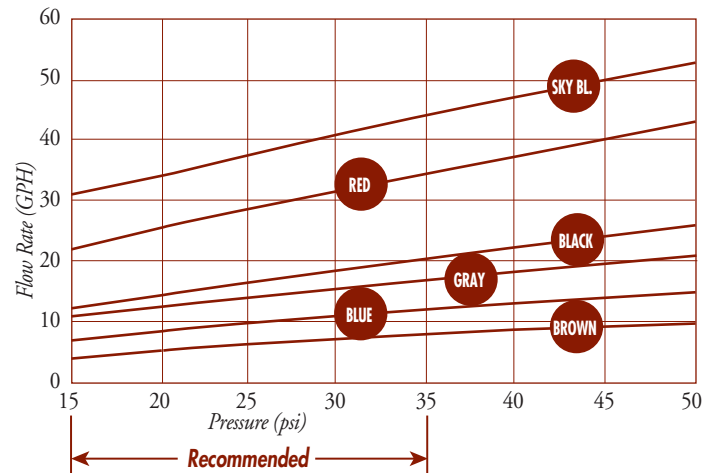
SUPERNET JR. Flow vs. Pressure
