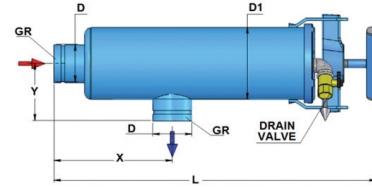
3" FILTER
