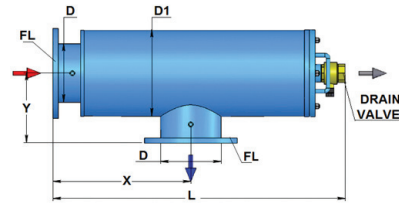
8" AND 10" FILTERS
