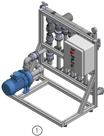
VALVE BRIDGE
