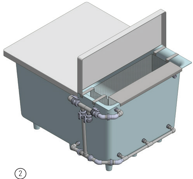
DISSOLVING TANK
